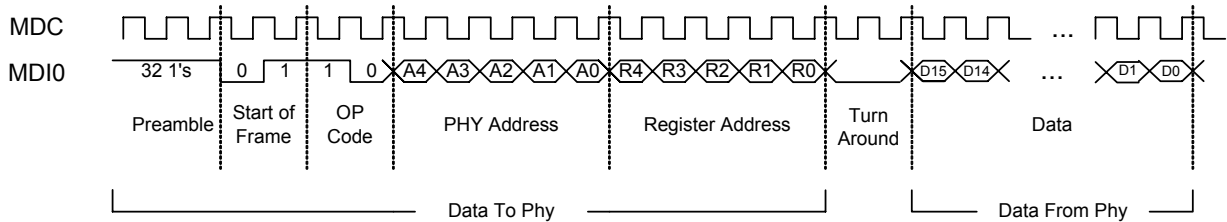
Figure 4.6 MDIO Timing and Frame Structure - READ Cycle
