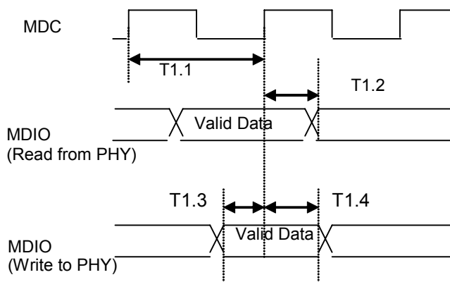
Figure 6.1 SMI Timing Diagram
